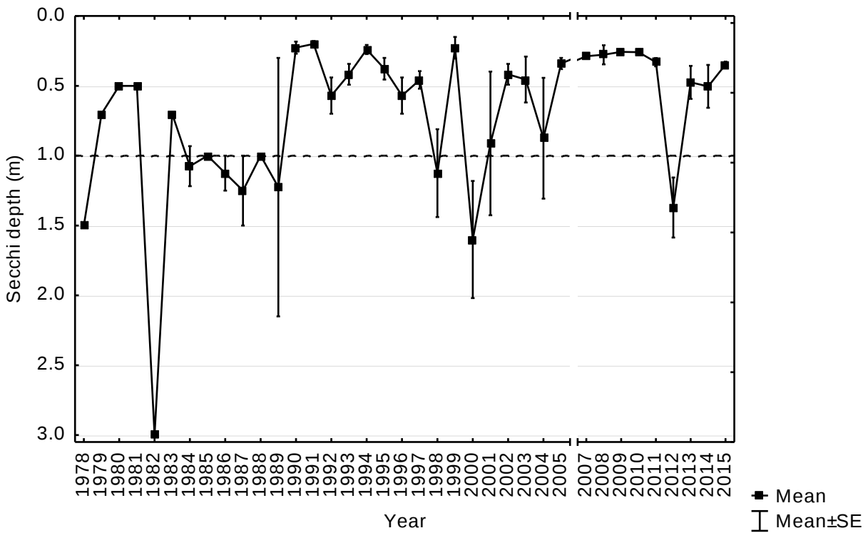
Figure 8. Growing season average Secchi depth, Lake Winona South (station 102)
