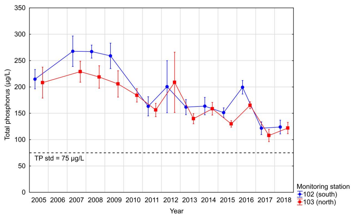
Figure 12. Growing season average phosphorus concentration, Lake Winona station 102 vs. 103, 2005–2018
