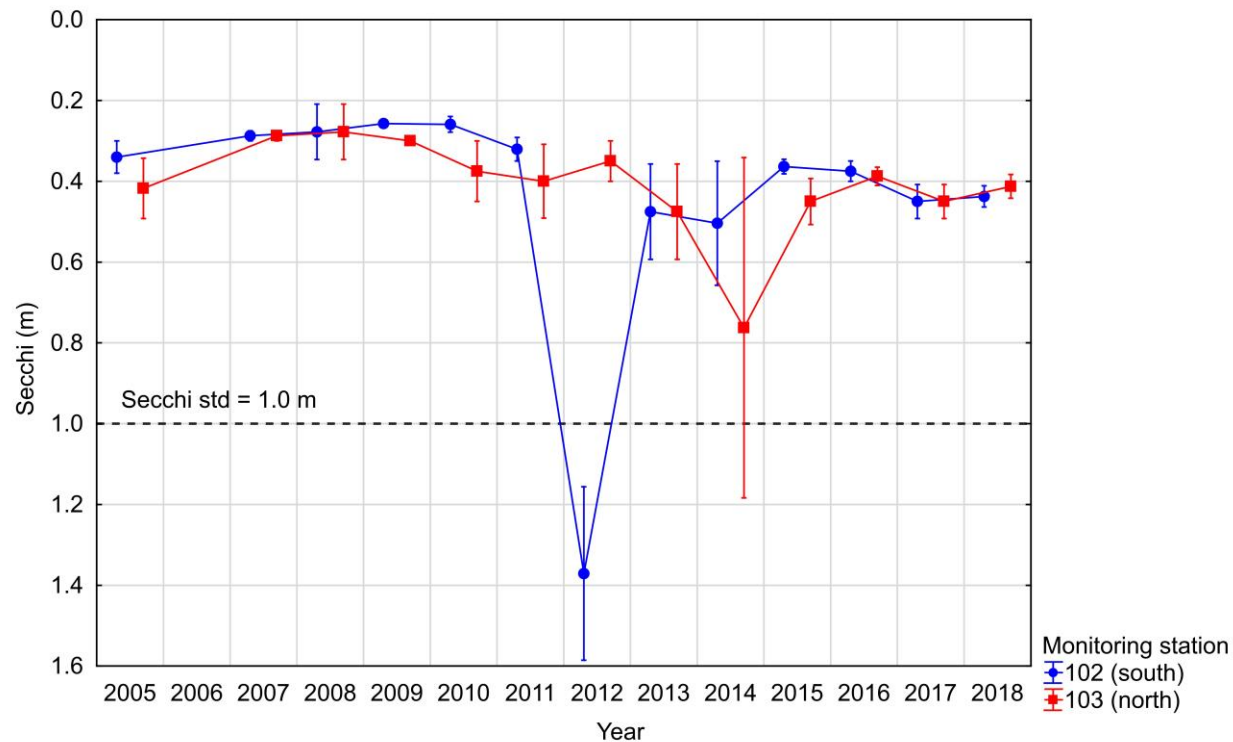
Figure 14. Growing season average Secchi depth, Lake Winona station 102 vs. 103, 2005–2018
