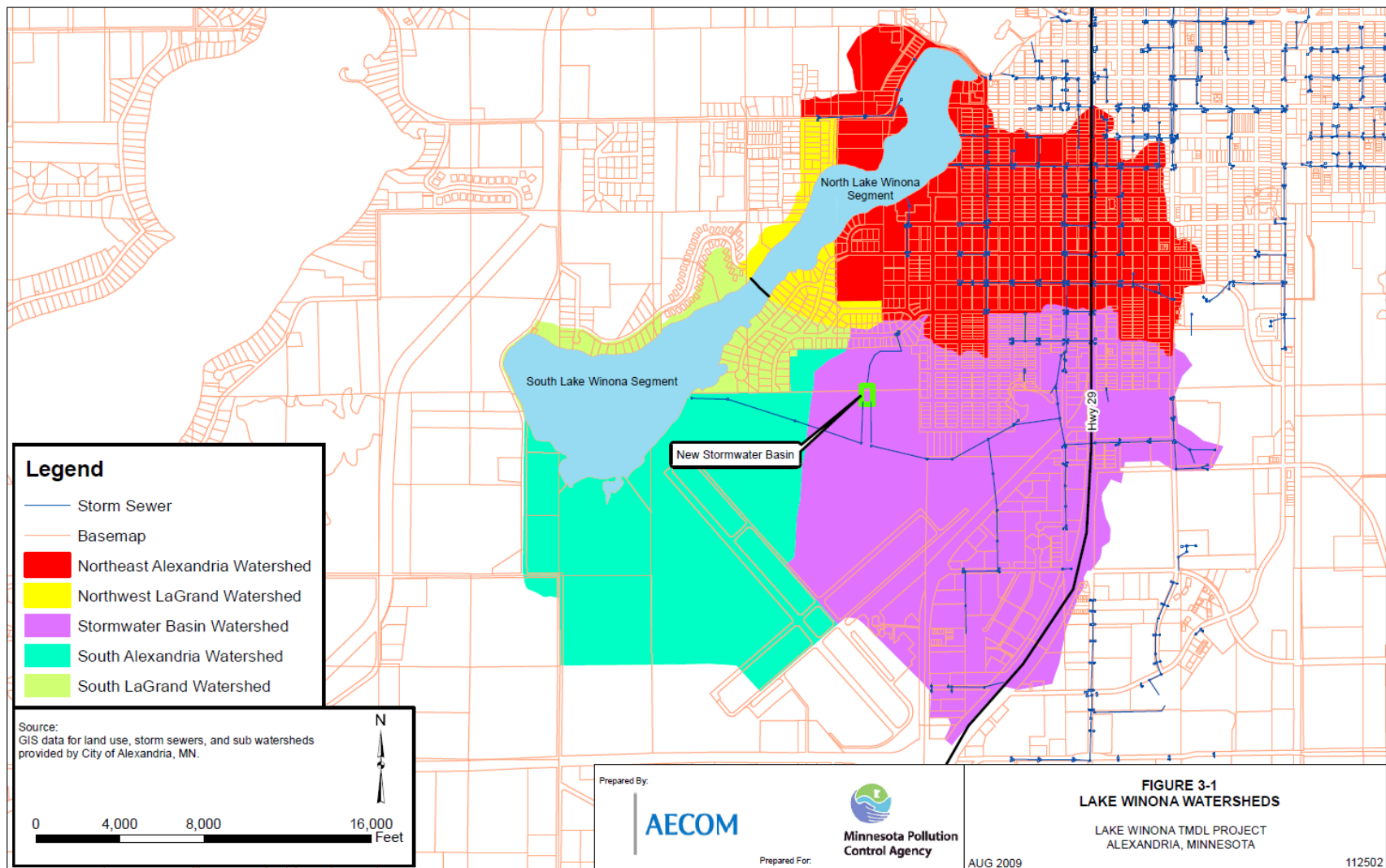
Figure 3. Lake Winona subwatersheds (AECOM 2009)
