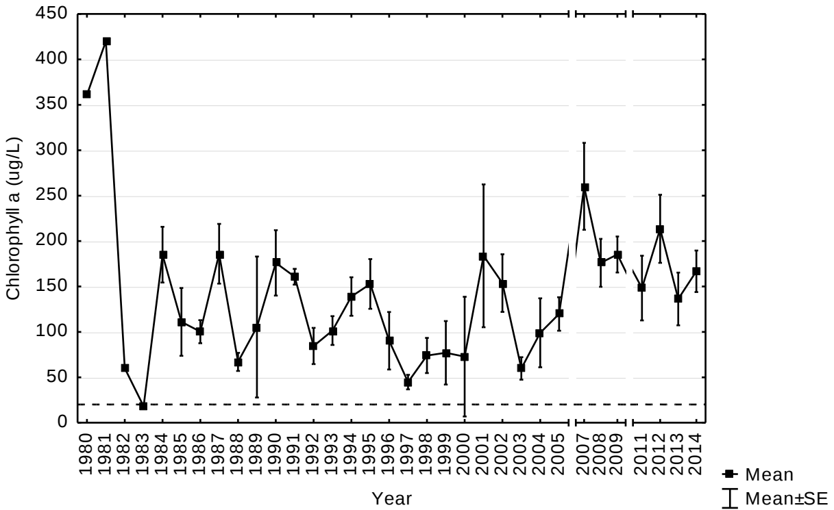
Figure 6. Growing season average chlorophyll-a concentration, Lake Winona South (station 102) Dashed line represents the site-specific standard of 20 µg/L
