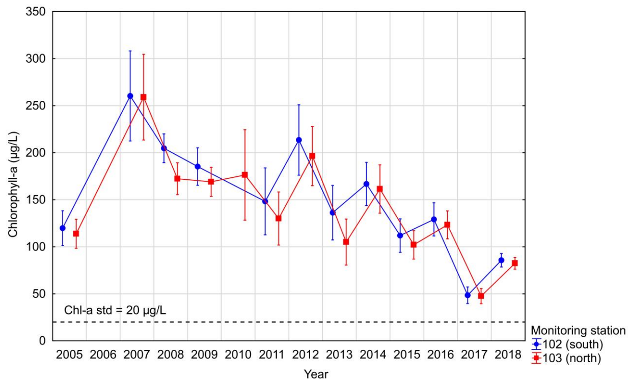
Figure 13. Growing season average chlorophyll-a concentration, Lake Winona station 102 vs. 103, 2005–2018
