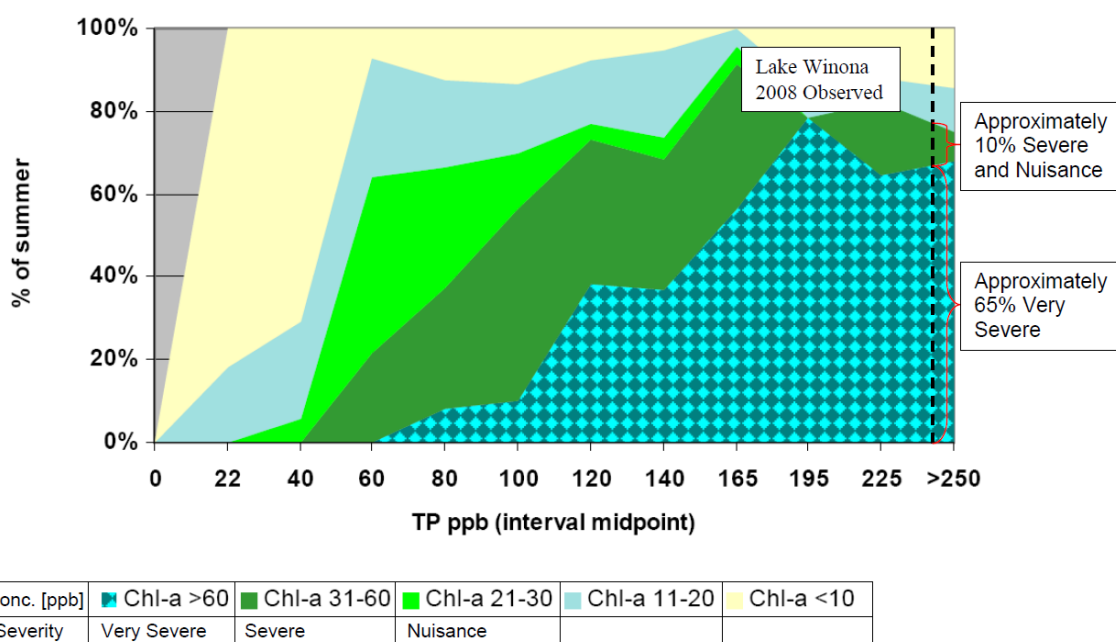
Figure 10. Algae bloom frequency for shallow lakes (Figure 12 in Heiskary and Lindon 2005)
