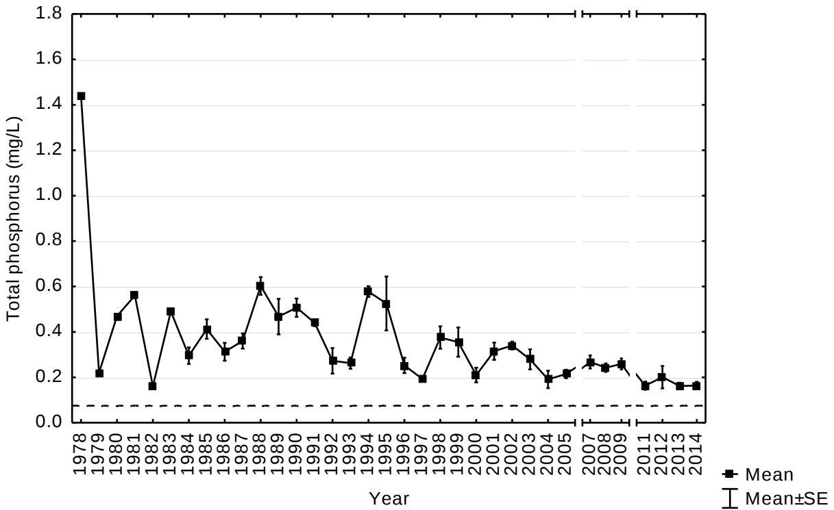
Figure 4. Growing season average phosphorus concentration, Lake Winona South (station 102) Dashed line represents the site-specific standard of 0.075 mg/L
