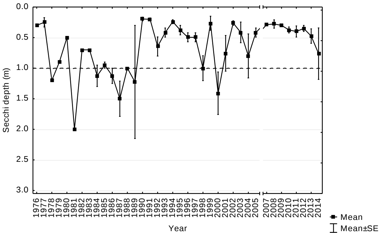
Figure 9. Growing season average Secchi depth, Lake Winona North (station 103)
