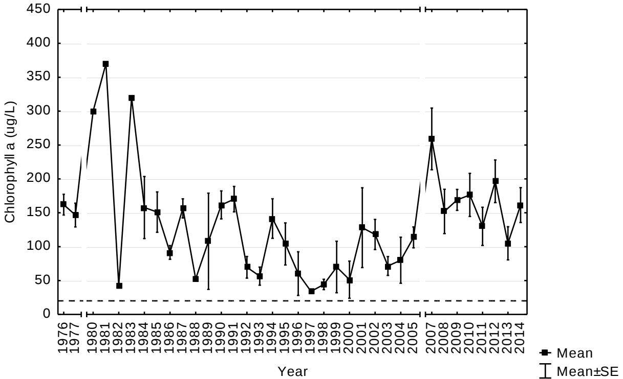
Figure 7. Growing season average chlorophyll-a concentration, Lake Winona North (station 103) Dashed line represents the site-specific standard of 20 µg/L
